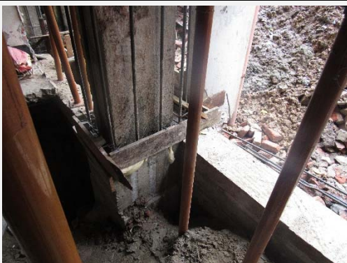
Supporting works
