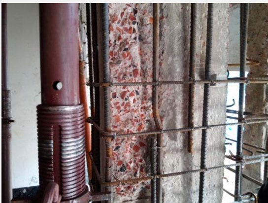
Retrofitting work
